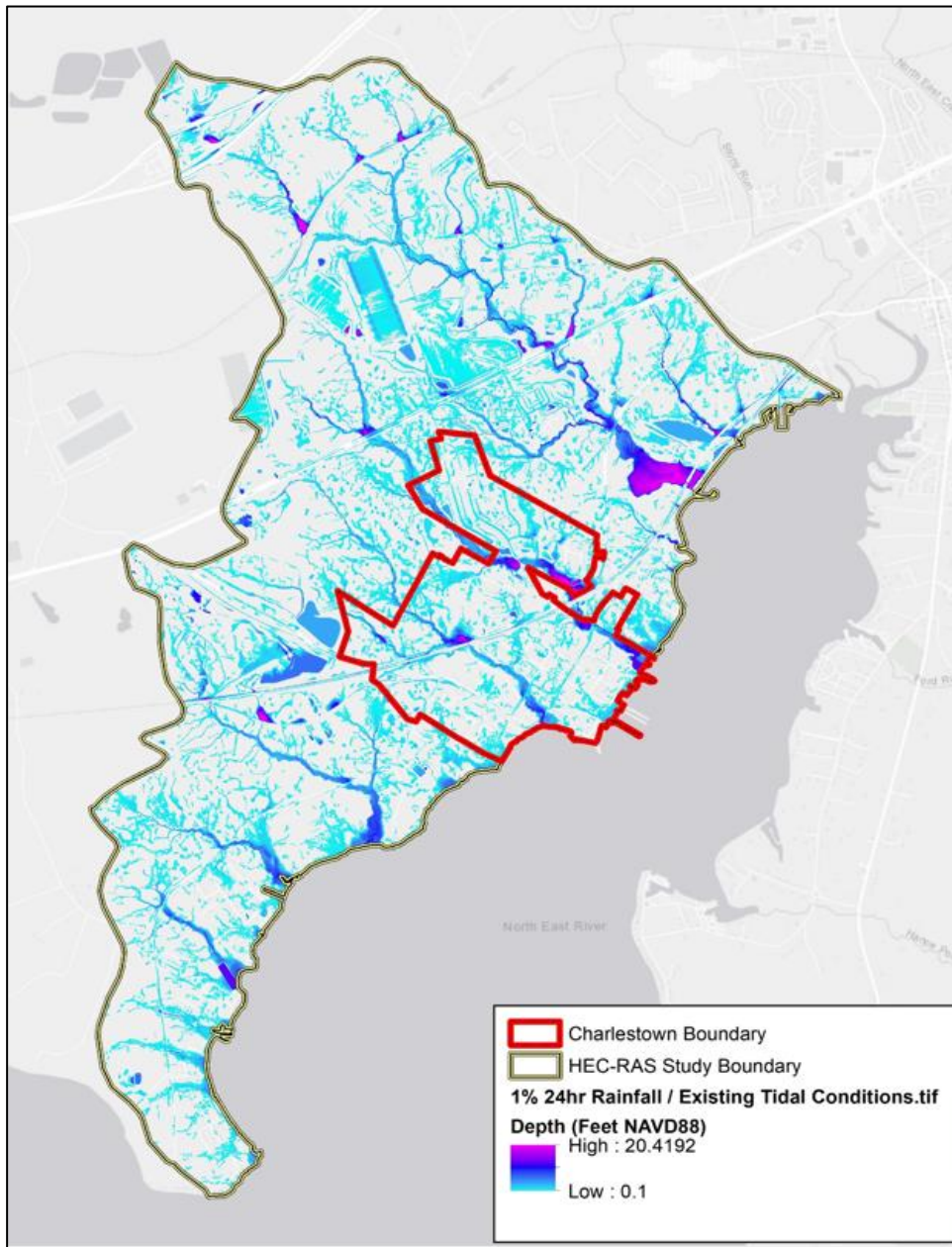
Figure 18: HEC-RAS Model Run – Entire Town
