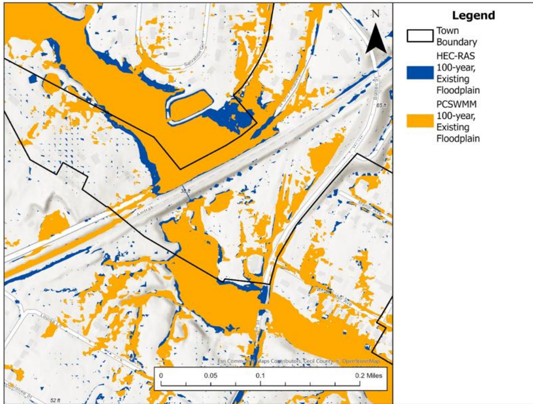
Figure 21: Comparison of the HEC-RAS and PCSWMM model at Old Philadelphia Road
