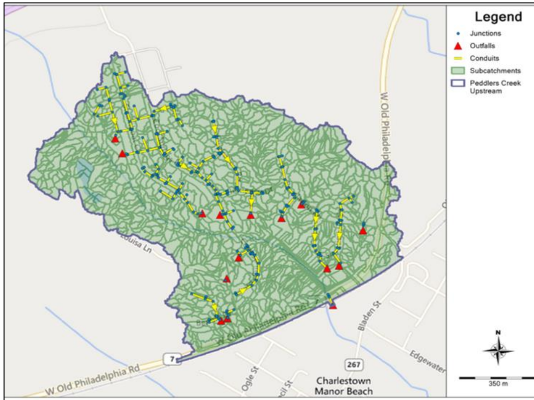
Figure 20: 1-D Stormwater network in Peddlers Creek Upstream PCSWMM model
